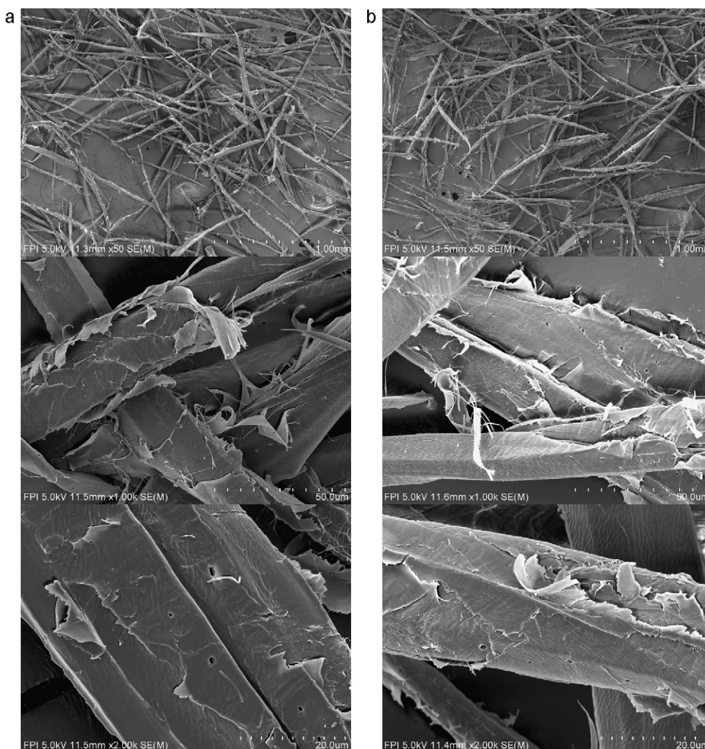
Fig. 4. SEM analysis of CTMP pulp fibers (a: CTMP1; b: CTMP3).
