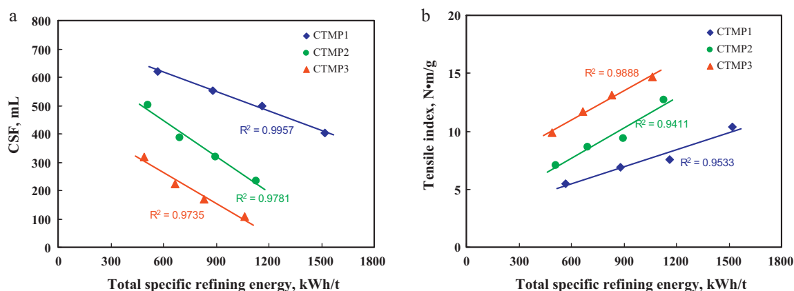
Fig. 2. Total specific refining energy vs. CSF (a) and tensile index (b) for CTMP pulps.
