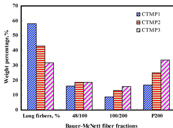
Fig. 3. Bauer-McNett fiber fraction of CTMP pulps that list in Table 4.
